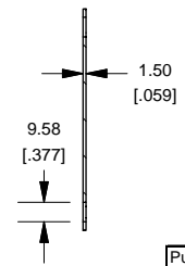
SECTION C-C Side View of Slot
