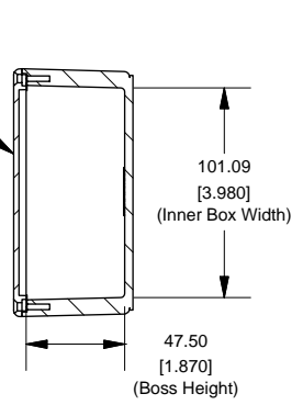
SECTION A-A End View of Assembly
